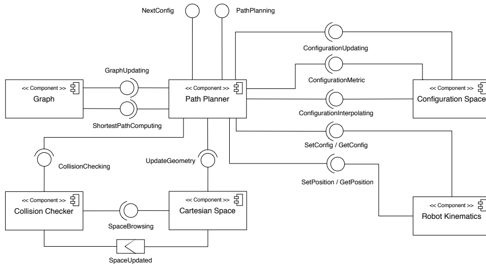
Fig. 1. The components system resulting from refactoring motion planning libraries
