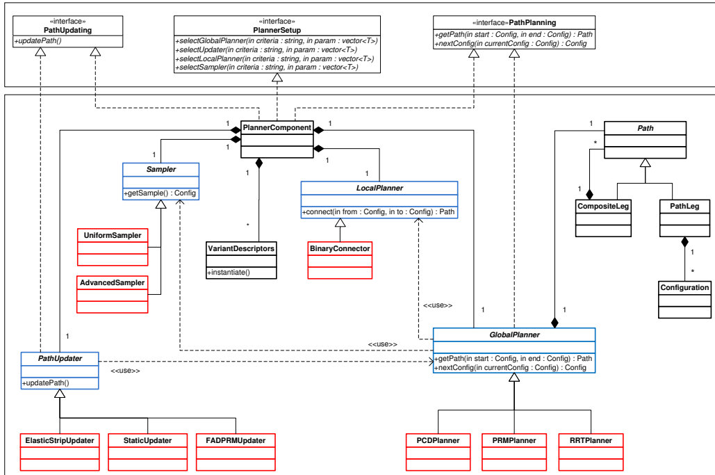
Fig. 2. The Path Planner Component Framework
