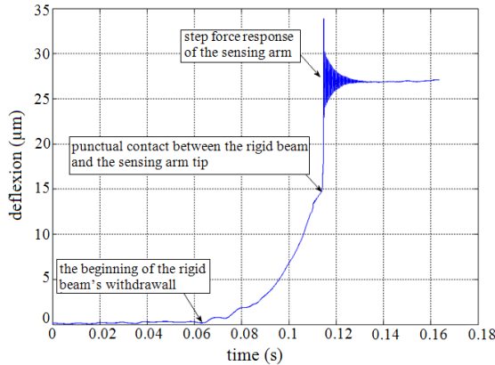
Fig. 9. Position response of the sensing arm tip to a 27μm thrust.
