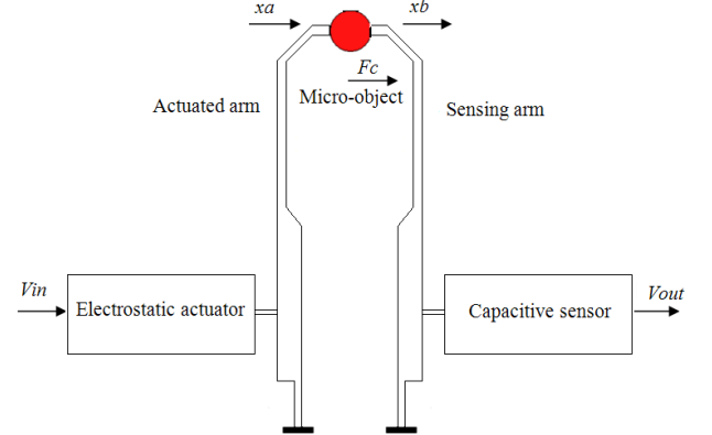
Fig. 3. System modelling.
