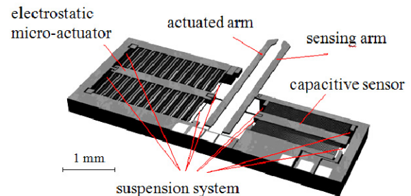
Fig. 1. Structure of the FT-G100 microgripper (FemtoTools GmbH).
