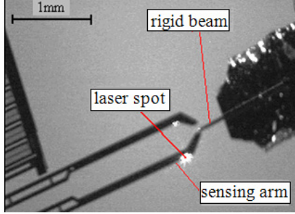
Fig. 8. Sensing arm excitation.
