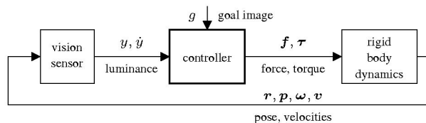
Fig. 2. Purely visual pose stabilization. We control in force and torque to stabilize a rigid body based only on the visual input y and \dot{y} , and a memorized goal image g taken at the desired pose. No inertial or velocity sensors are used.
