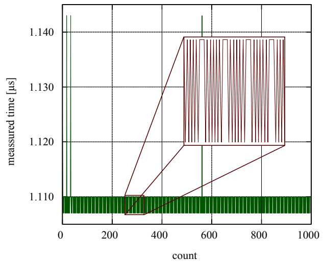
Fig. 11. Jitter measurement
