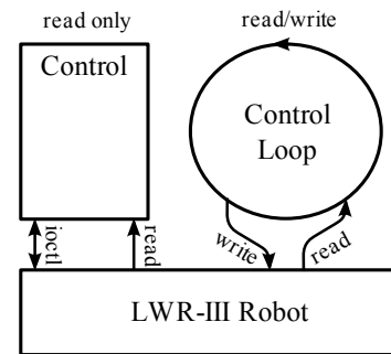
Fig. 6. POSIX Device Driver mapping
