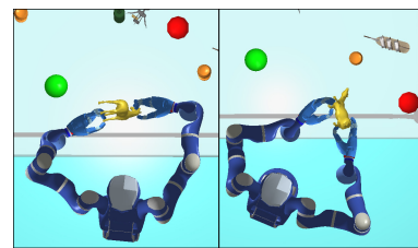
Fig. 7. Example of computed exchange positions for different initial (red) and final (green) object poses, taking into account the cost to minimize and obstacle collision avoidance.
