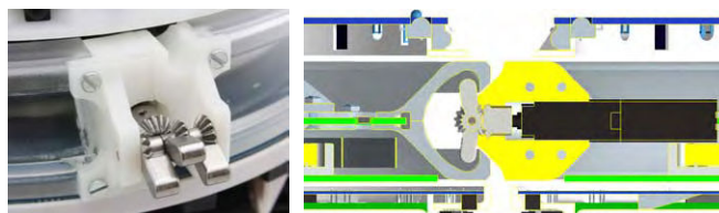
Fig. 5: Attachment device and mechanism.
