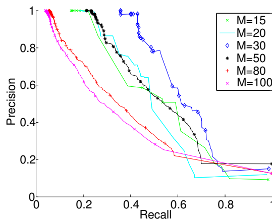
(b) Precision-recall curve on the simulation sequence. Different values of M were tested. Larger contexts are beneficial when common words are avoided when computing virtual locations.
