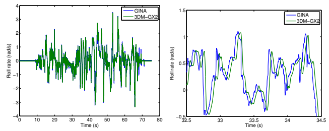
Fig. 6. Comparison of gyro output between GINA and 3DM-GX2
