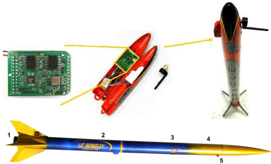
Fig. 2. The original rocket containing GINA sensors (above) has evolved to the rocket shown on the bottom, using the WARPWING platform for 3 axis inertial attitude feedback control.
