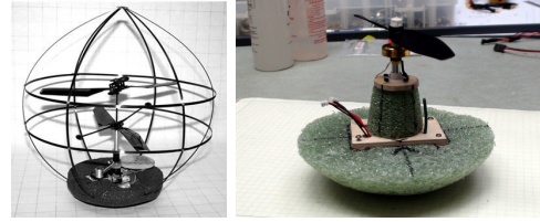
Fig. 12. The hopping rotochute developed at GATEch uses WARPWING as its flight controller. The software interface was rewritten to fit in to the existing MATLAB framework, while the rest of the WARPWING system remained unchanged. This allowed for quick development of the mini rotochute, shown at right.
