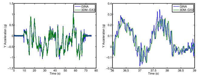
Fig. 7. Comparison of acceleration output between GINA and 3DM-GX2
