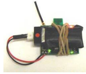
Fig. 15. This small lightweight vibration sensor is designed from the schematic level on up using the WARPWING system as a base, but replacing the accelerometer with one far more sensitive. It is intended to be used in a network to sense footsteps and localize them using time difference of arrival.
