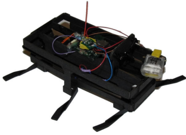
Fig. 14. DASH, a small, lightweight crawling robot developed at UC Berkeley, uses the WARPWING system to measure inertial rates and motor back EMF for dynamic analysis and control.
