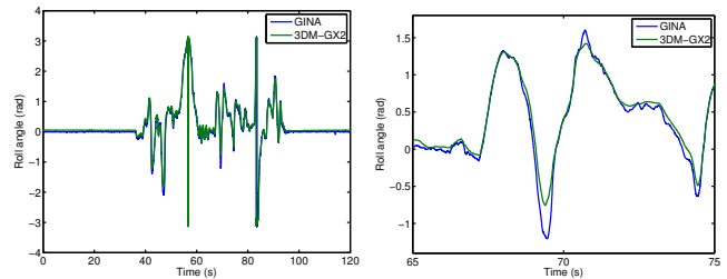
Fig. 8. Roll angle estimate comparison. GINA and 3DM-GX2 agree closely in their state estimates.
