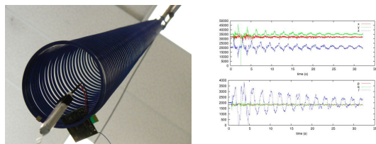
Fig. 11. Inertial data collected from a GINA mote mounted on a coiled spring, demonstrating both oscillatory rotation and translation. Data courtesy Thomas Watteyne.
