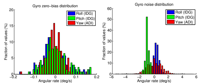
Fig. 4. The variation of the gyro zero-bias for a single board across 150 runs over 5 days is shown in the graph on the left for each of the three axes. The graph on the right shows the zero-rate gyro outputs over 2000 measurements during a single run. The bias offsets are clearly visible in the right graph, as well as a notable difference in performance between the two gyros.
