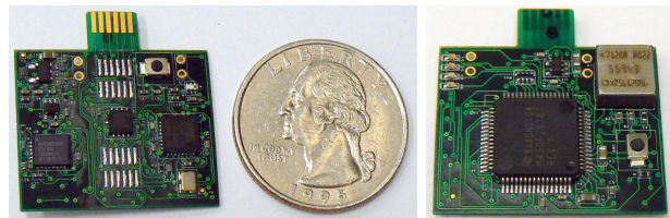
Fig. 1. GINA provides inertial sensing, processing, control, and wireless communication on a board smaller and lighter than a US quarter.
