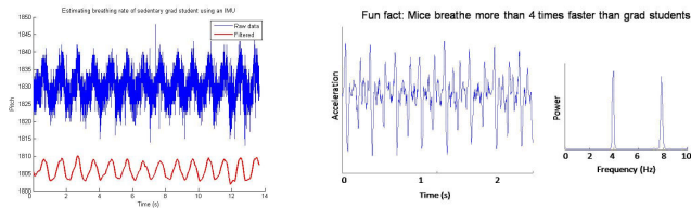
Fig. 10. Inertial data collected from GINA notes mounted on mammals is used to calculate sedentary breathing rates. Data courtesy Subramaniam Venkatraman.
