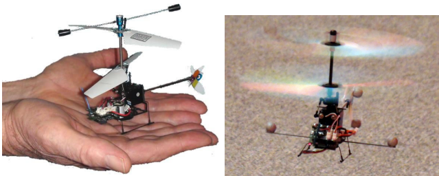
Fig. 3. GINA is mounted onto an off the shelf miniature coaxial helicopter, using a daughter board to connect to the actuators. On the right, this helicopter is shown using the WARPWING system to autonomously hover.
