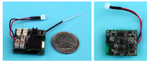
Fig. 5. A daughter board for the GINA mote brings PWMs out to connectors for servos, uses other PWMs for brushed motor controllers, and includes additional sensors such as a battery fuel gauge, GPS receiver, and vision processors.
