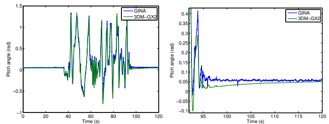
Fig. 9. Pitch angle estimate comparison. The noisier GINA estimate also allows a much shorter settling time than the 3DM-GX2.
