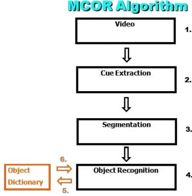
Fig. 1. Flow of MCOR framework: (From top to bottom) (1.) Get frame from video, (2.) extract cues from the image, (3.) segment the image and associate extracted cues with a segmented region, (4.) recognize objects based on dictionary, (5.&6.) update object dictionary based on the recognized objects, search image again with updated dictionary including updated visual description of object.
