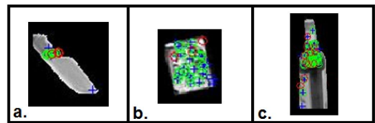
Fig. 10. Examples of SIFT models extracted from one training example of (a.) a knife, (b.) a cereal box, and (c.) a wine bottle. Green circles indicate keypoints used in a match, red circles indicate outliers, and blue plus signs indicate matches from nearest neighbors.
