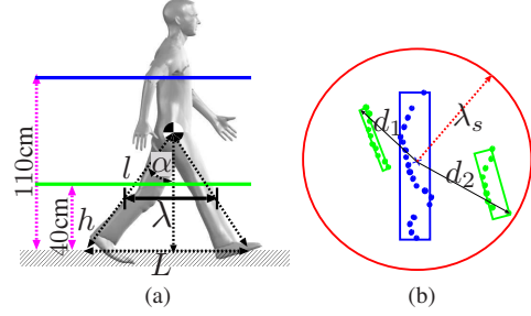
Fig. 2: Walking model and layer fusion: (a) separation between legs \lambda at sensor height h , and (b) search area for association.
