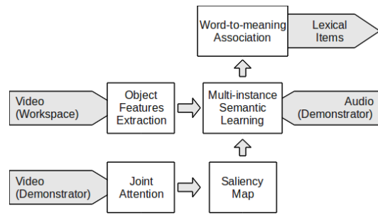
Fig. 1. General model overview.
