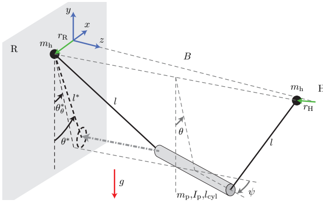
Fig. 2. T-pendulum setup: cylindrical pendulum object of mass m_p , length l_{cyl} and inertia I_p actuated by a human H and a robot R through the handle masses m_h .
