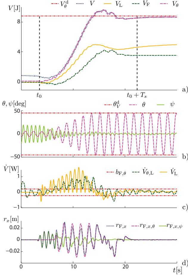
Fig. 5. Example trial of a robot follower cooperating with a robot leader in simulation for initial conditions \theta_{0,2} = 5.7^\circ , \psi_{0,2} = 19.4^\circ and a desired energy specified by \theta_V^d = \frac{\pi}{4} : (a) energies V , (b) angles \theta and \psi , (c) actual energy flow of leader \dot{V}_L and estimation \dot{V}_{\theta,L} directed towards the \theta -oscillation, (d) composition of follower trajectory r_x .
