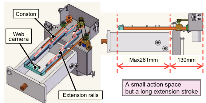
Fig. 7. The structure of extensible arm.
