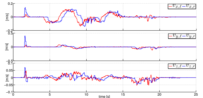
Fig. 8: Local and remote robots linear velocities.
