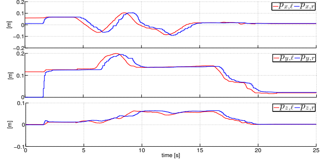
Fig. 5: Local and remote robots positions.
