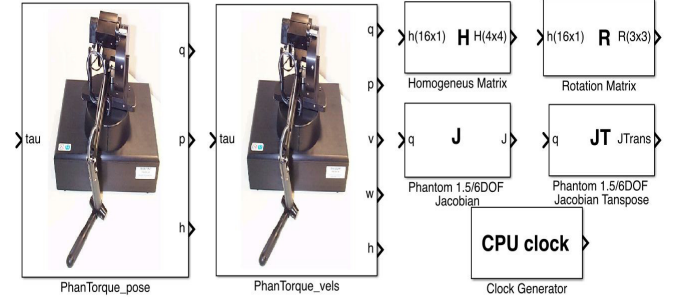
Fig. 3: PhanTorque library
