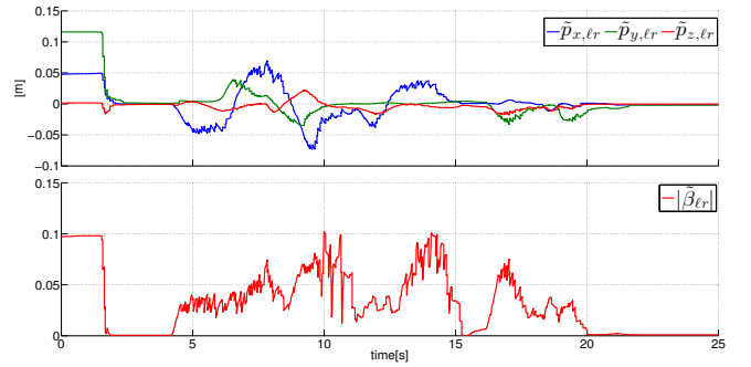
Fig. 7: Teleoperation system pose errors.
