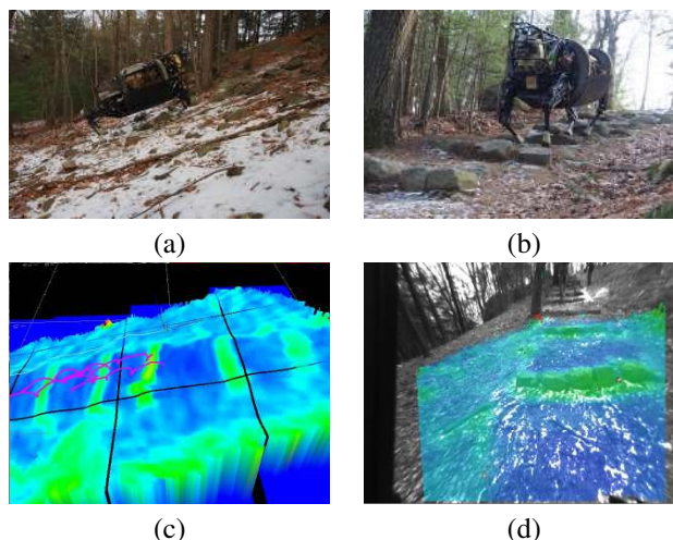
Fig. 1. (a) and (b) show the LS3 vehicle walking up and down a set of stairs on a forest trail; (c) shows the 2D terrain map color coded by step height (from flat (blue) to moderate (green) to high (red)), with the foot traces in magenta; and (d) shows the backprojection of the map overlaid on the left stereo image.
