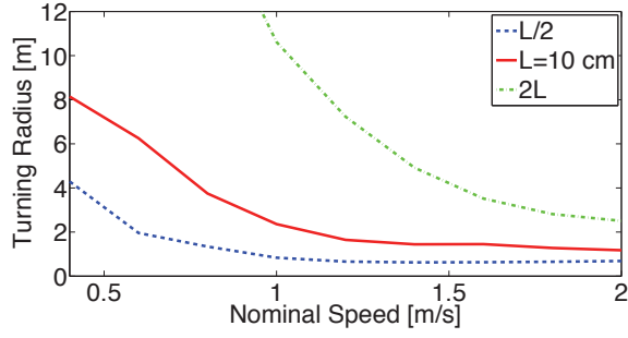
Fig. 8. From simulation, aerodynamic steering is more effective for small robots.
