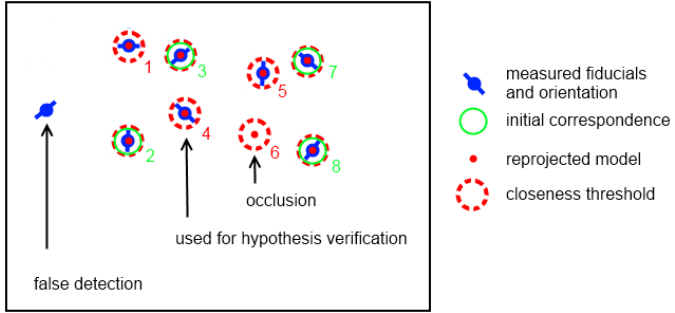
Fig. 6: Fiducial correspondence on the image plane, showing initial correspondence, model rejections, an occlusion and a false detection.
