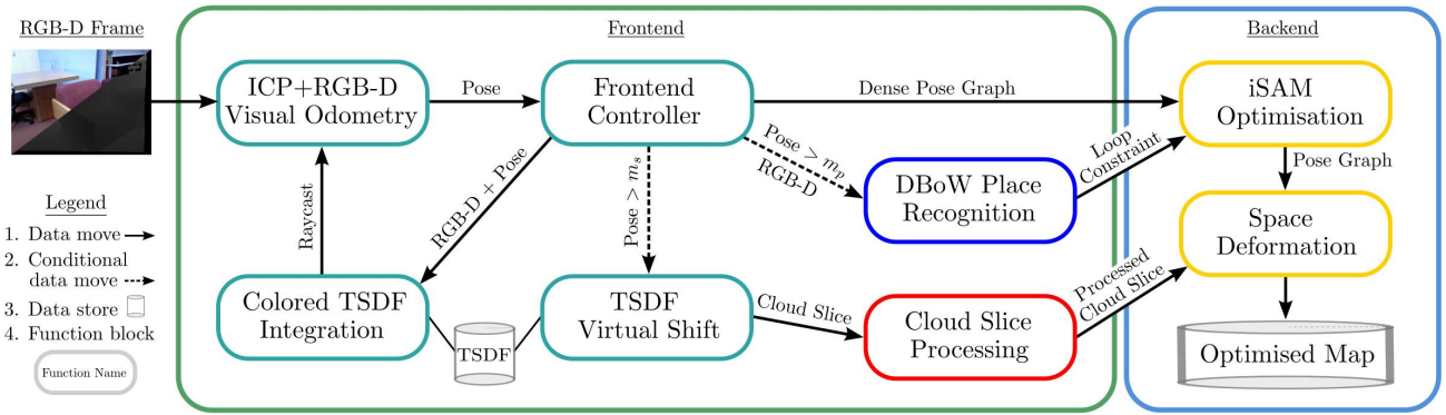
Fig. 2. System architecture diagram. Differently colored function blocks are executing asynchronously in separate CPU threads. The m_s quantity denotes the volume shifting threshold and m_p denotes the place recognition movement threshold.
