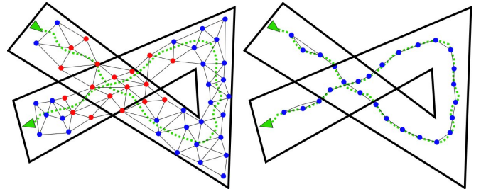
Fig. 4. Two-dimensional example of deformation graph construction. On the left a spatially-constrained graph is constructed over a pre-loop closure map suffering from significant drift. The nodes highlighted in red are connected to nodes which belong in potentially completely unrelated areas of the map. On the right our incremental sampling and connectivity strategy is shown (two-nearest neighbours for simplicity) which samples and connects nodes along the dense pose graph, preventing unrelated areas of the map being connected by the deformation graph.
