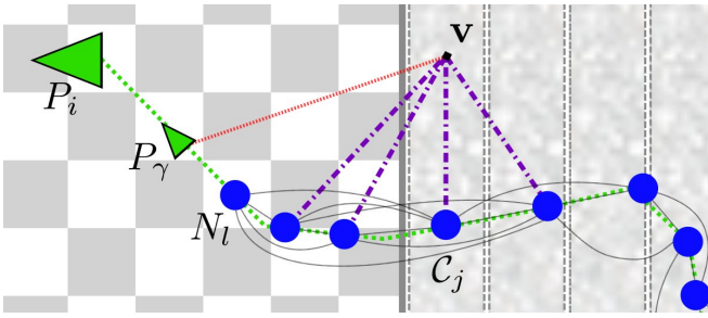
Fig. 3. Two-dimensional example showing the current position of the TSDF shifting volume as a checkerboard pattern and the previously extracted cloud slices as textured columns. Also shown is the dense pose graph as small green points as well as a pose P_\gamma which caused a volume shift. The association between P_\gamma and the extracted cloud slice is shown with a dotted red line. A k = 4 connected sequential deformation graph is also shown, demonstrating the back-traversal vertex association algorithm on a random vertex \mathbf{v} .
