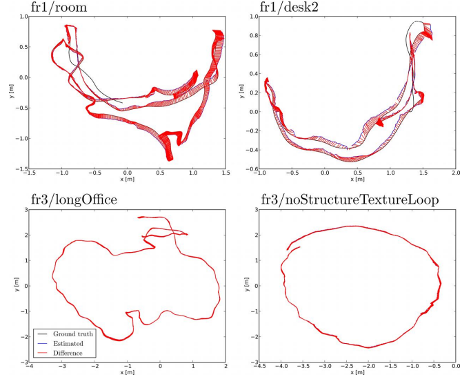
Fig. 5. Absolute trajectory errors on the four evaluated RGB-D benchmarks using the hessian uncertainty estimate.
