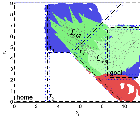
Fig. 7. Transition funnels for \mathcal{L}_{56} and \mathcal{L}_{67} (green). \mathcal{L}_5^c and \mathcal{L}_7^c are shaded red and \mathcal{L}_6^c is shaded blue.
