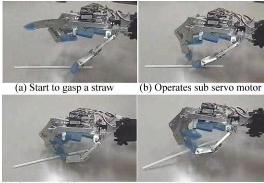
Figure 7. Situation of manual operate mode (tip a straw)
