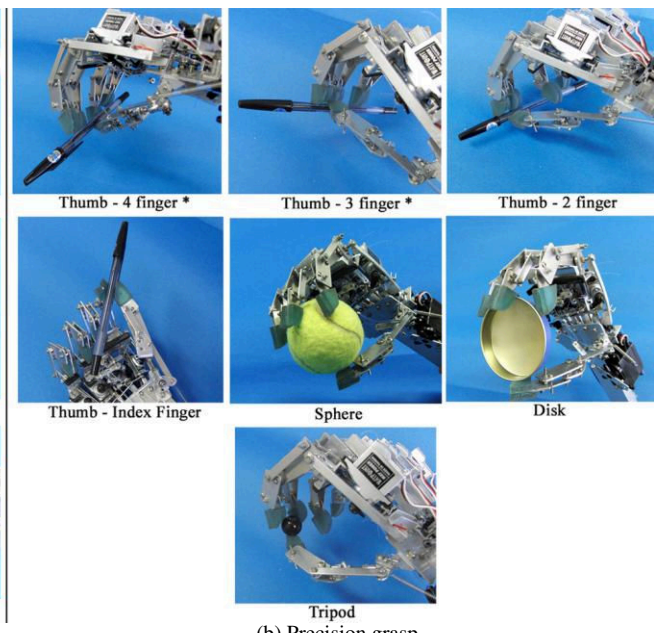
Figure 8. Result of grasping experiment of new model based on Cutkosky's taxonomy [22]
