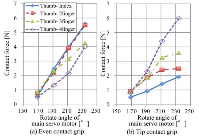
Figure 14. Results of contact force at grip type
