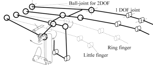
Figure 5. Movement motion of the palm part
