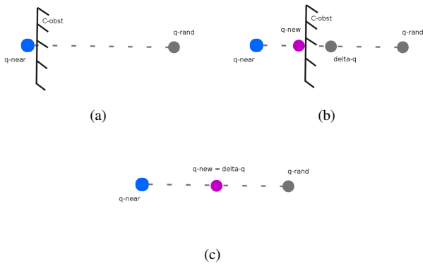
Fig. 1. Possible outcomes during RRT expansion: (a) null expansion of q_{near} against C_{obst} ; (b) partial expansion of q_{near} which collides with C_{obst} before reaching \Delta q ; and (c) full expansion of q_{near} to \Delta q .
