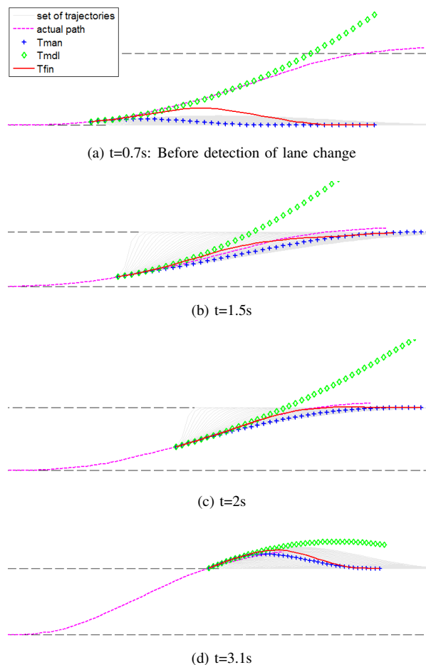
Figure 7: Example of predictions for a left lane change
