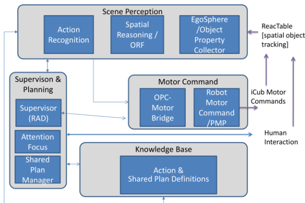
Fig. 2. Control Architecture for cooperative interaction. Spatial location of objects on ReacTable communicated to Object Property Collector which stores the state of the world. Spatial reasoning detects object movement and spatial relations among them providing the required information for Action Recognition . Supervision and Planning monitors interaction, focuses gaze attention on linguistic references, and manages joint/shared plan execution. Shared plans and action definitions are stored for long term use in Knowledge Base . Motor command monitors manipulation of object predicates transformed to motor space using passive motor paradigm (PMP). See text for details.
