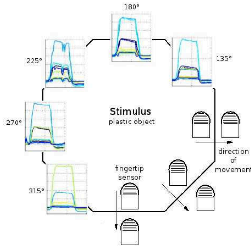
Fig. 2. Data collection for an edge stimulus over a range of orientations and positions. The object was turned at every 5 deg steps and the sensor was tapping along 18 mm at 0.2 mm steps for each angle. For visualisation, we show only five examples from a total of 72 angle and 18 position classes.
