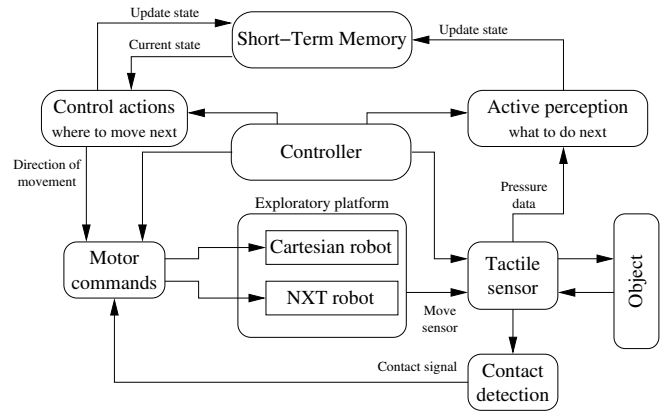
Fig. 4. Sensorimotor architecture developed for applying active Bayesian perception to an online task. The tactile sensor provides the feedback from the world, whilst the mobility in x -, y - and z axes is provided by the robotic platform. The what to do next and where to move next decisions are implemented by the 'active' perception and 'control actions' modules, respectively.
