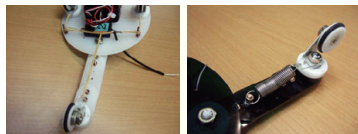
Fig. 13. Modification of the elastic elements
