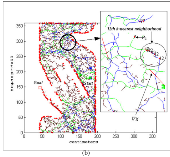
Fig. 5. a) Sensor-based RRT algorithm; b) Sensor-Based BNM algorithm. Each red dot represent a point cloud obtained by the 3D sensors.
