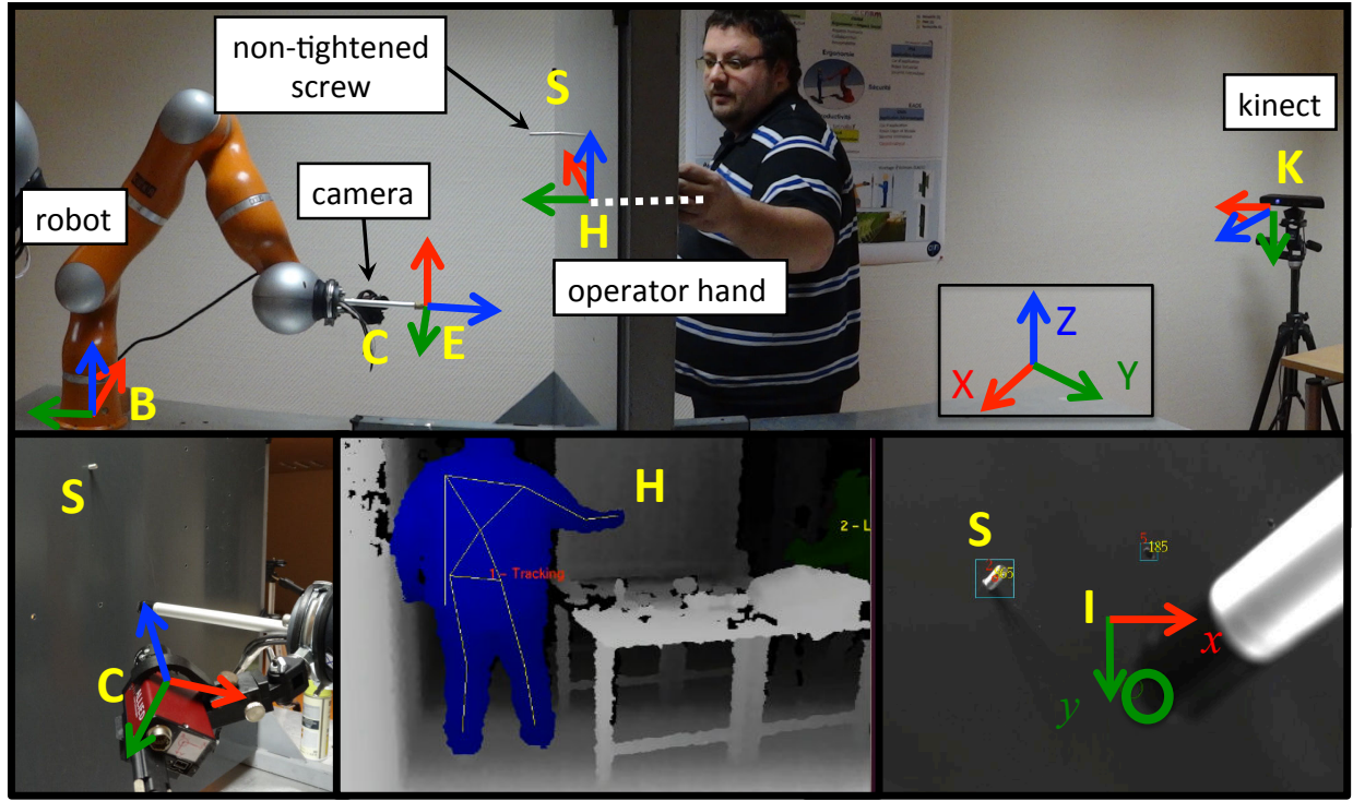
Fig. 1. Reference frames used in this work. Top: experimental setup. Bottom left: view of the camera and effector. Bottom center: Kinect image. Bottom right: camera image.
