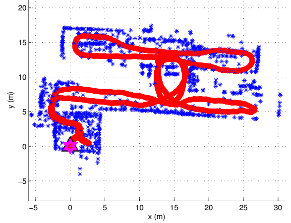
Fig. 1. The overhead x-y view of the IMU-Kinect 3D trajectory and the point features estimated by the OC-MSC-KF SLAM.
