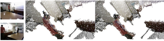
Fig. 3. Left: When a naive nearest-neighbor metric is applied, two sides of an object will be drawn toward each other, often at the expense of violating free space. Right: Our occlusion-aware energy term is able to recover from many of these situations.
