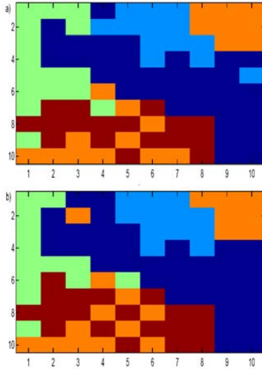
Fig. 3. Mapping the MaRC bank onto a SOM. The colours navy blue, sky blue, green, orange, and brown indicate that the corresponding neuron belongs to NN_1, NN_2, NN_3, NN_4 and NN_5 , respectively. In a) the color indicates that the corresponding NN has minimum error (desired network selection). b) shows the choice of the cluster pointers. Note that the selection of the cluster pointers match very closely to the NN selection.
