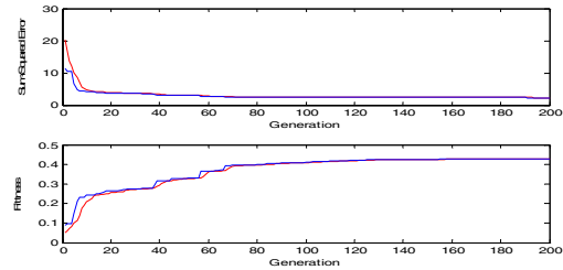
Figure 2. Sum-squared error and fitness curve of GA
