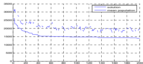
Figure 4. The solution and population curve
