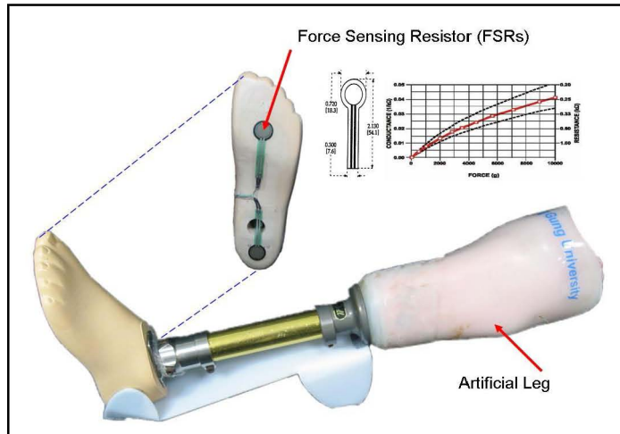
Figure 2. Force sensing resistors on artificial leg
