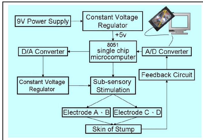
Figure 3. Flow chart of control signal in the subsensory stimulation unit
