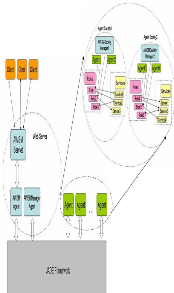
Figure 1. AWSM Framework Architecture
