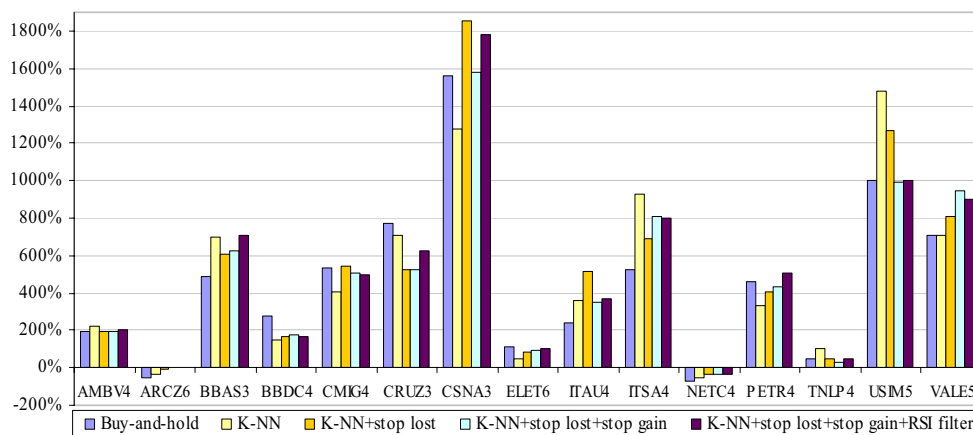
Figure 2. Results compared to buy-and-hold estategy
