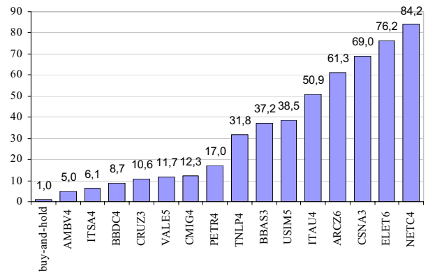
Figure 3. Results for a hypothetical classifier versus buy-and-hold strategy
