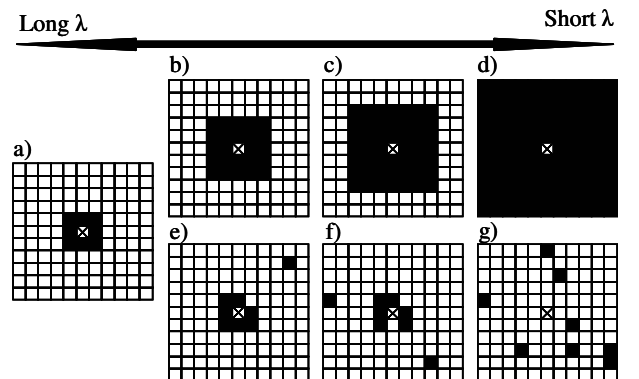
Fig. 1. Schematic diagram of representative types of mating neighborhoods for a given cell (x). Mating neighborhoods comprised the cell itself as well as those shown in black. a) 3 \times 3 local neighborhoods, b-d) local neighborhoods with increasing relative neighborhood size ( \delta ), and e-g) 3 \times 3 local neighborhoods with increasing probability of long-distance interactions ( p ). Characteristic path length ( \lambda ) decreases from left to right.
