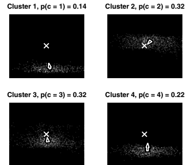
Fig. 7. Relative spatial distributions of the four input clusters. White indicates high occurrence, black low occurrence. The cross in the center represents the object location. The arrow is the action taken by the agent, when the input is equal to the cluster centroid. The arrow originates at the median of the relative x - and y - coordinates of the cluster.
