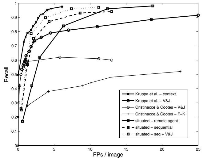
Fig. 10. FROC-curve for the results on the FGNET face-detection task from different studies.
