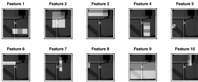
Fig. 5. The ten features evolved for the mug-detection task, shown within the scanning window (white box). The white cross indicates the gaze location.
