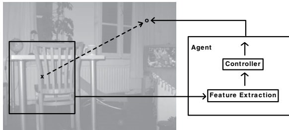
Fig. 1. Illustration of a step in the situated object detection process. The agent obtains sensory inputs by extracting features from a square window of gray values in the image. This window, referred to as the fovea, is centered at the gaze location (‘x’). The agent’s controller maps the sensory inputs to a gaze shift in the image (dashed), determining the next gaze location (‘o’).
