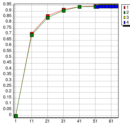
Fig. 6. SVM performance on subsequent collections of PCs.
