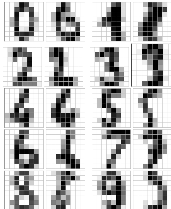
Fig. 2. Training data examples.
