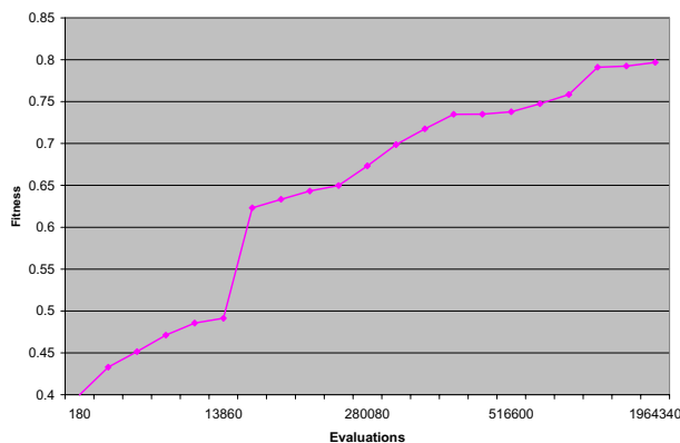
Fig. 4. The fitness trend of the hill climber, which developed a high performance agent within less than 2 million evaluations. These results scored even better than the co-evolution, resulting in a more efficient agent in less time.
