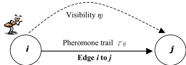
Figure 3. Design outline of proposed ant algorithm hyper-heuristic [23]
