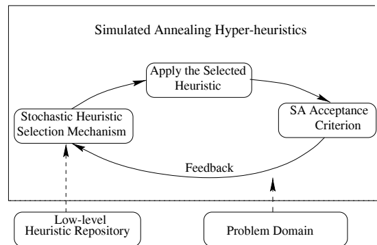
Fig. 1. A diagram of the simulated annealing hyper-heuristic
