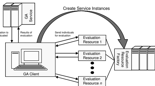
Fig. 4. The Implementation of the Optimisation Framework
