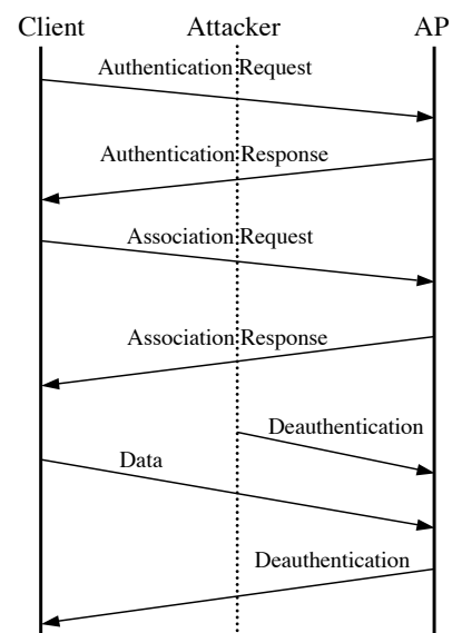
Fig. 1. Deauthentication Attack [5]
