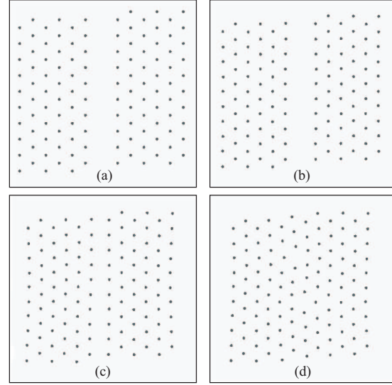
Fig. 7. Simulation results for maintenance and unification with 120 robots under no environmental constraint ((a) t = 0[\text{sec}] , (b) t = 5[\text{sec}] , (c) t = 14[\text{sec}] , (d) t = 20[\text{sec}] )
