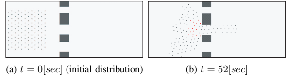
Fig. 11. Simulation results for flocking without partition capability
