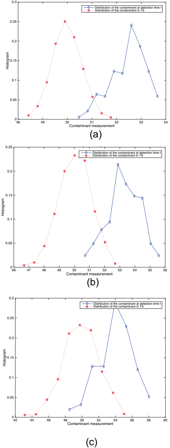
Fig. 6. Distribution of the contaminant measurement at detection time \hat{T} for all the experiments where the contaminant has been correctly detected and isolated (blue solid line) and distribution of the contaminant measurements up to time t_0 = 1000 (i.e., the training set) for the zone where the contaminant source has been inserted (i.e., the source zone). The considered scenario is number 1 and \Gamma = 2.5 . Figure (a), (b) and (c) refer to \sigma = 0.5 , \sigma = 1 , and \sigma = 2 , respectively.
