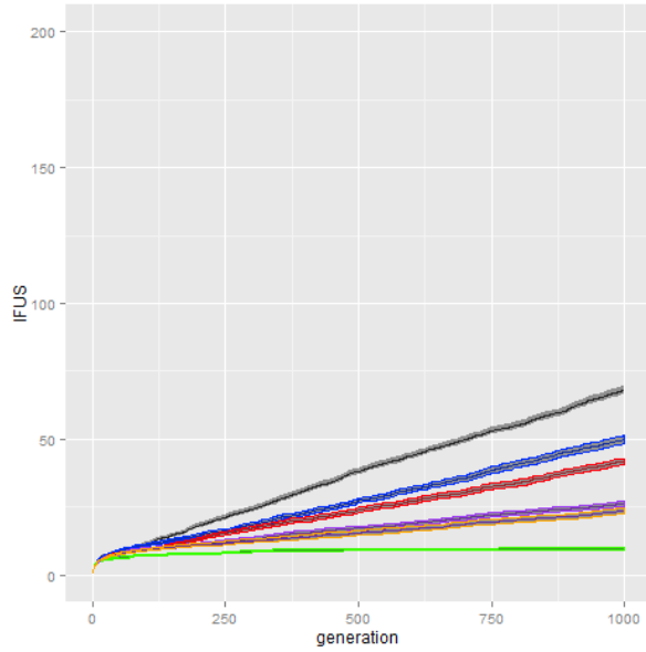
Figure 8. The influence of niching coefficients on complexification. Black: 1.0; blue: 0.5; green: 2.0; red: -0.5; purple: -1.0; orange: -2.0.
