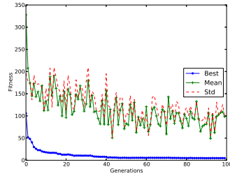
Fig. 15: 0,53% nanotubes, evolve minimum difference on 2 output pins, 1 single input.
