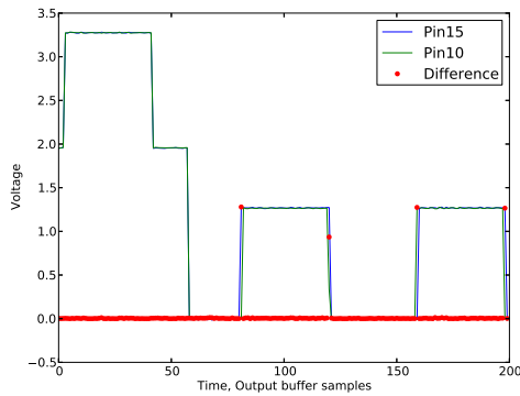
Fig. 26: 5,00% nanotubes, example with 2 inputs, evolve min difference. Input pin 4: 3208 Hz, duty cycle 94%; Input pin 13: 400 Hz, Duty cycle 79%, Output pins: 15, 10.
