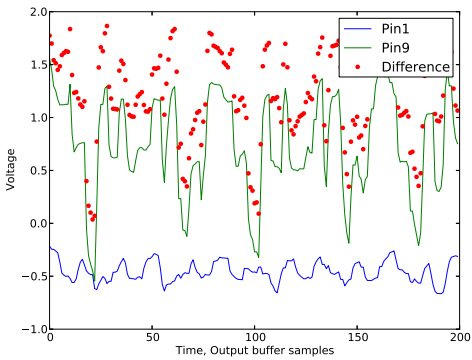
Fig. 29: 0,53% nanotubes, example with 10 inputs, evolve max difference. Input pins (pin#, frequency Hz, duty cycle %): (12, 14190, 13), (8, 22055, 30), (7, 15255, 57), (0, 13302, 100), (11, 15089, 69), (5, 6322, 21), (10, 9437, 72), (14, 7471, 55), (13, 15197, 17), (15, 9928, 29). Output pins: 1, 9.
