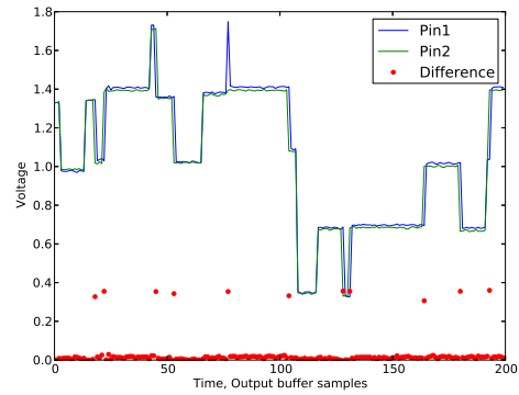
Fig. 27: 5,00% nanotubes, example with 10 inputs, evolve min difference. Input pins (pin#, frequency Hz, duty cycle %): (13, 1976, 78), (9, 3996, 11), (10, 1984, 10), (7, 657, 71), (11, 866, 13), (15, 663, 93), (12, 2060, 41), (6, 24500, 100), (14, 1462, 94), (8, 12910, 100). Output pins: 1, 2.
