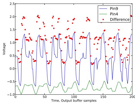
Fig. 28: 0,53% nanotubes, example with 2 inputs, evolve max difference. Input pin 10: 9595 Hz, duty cycle 79%; Input pin 8: 20299 Hz, Duty cycle 91%, Output pins: 9, 4.
