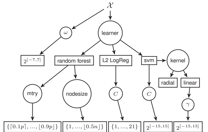
Fig. 1. Joint parameter space of the second experiment. Circles denote variables, rectangles denote values of numerical and discrete parameters, arrows denote the hierarchic structure. Here n denotes the number of observations, p the number of features in the respective data set.
