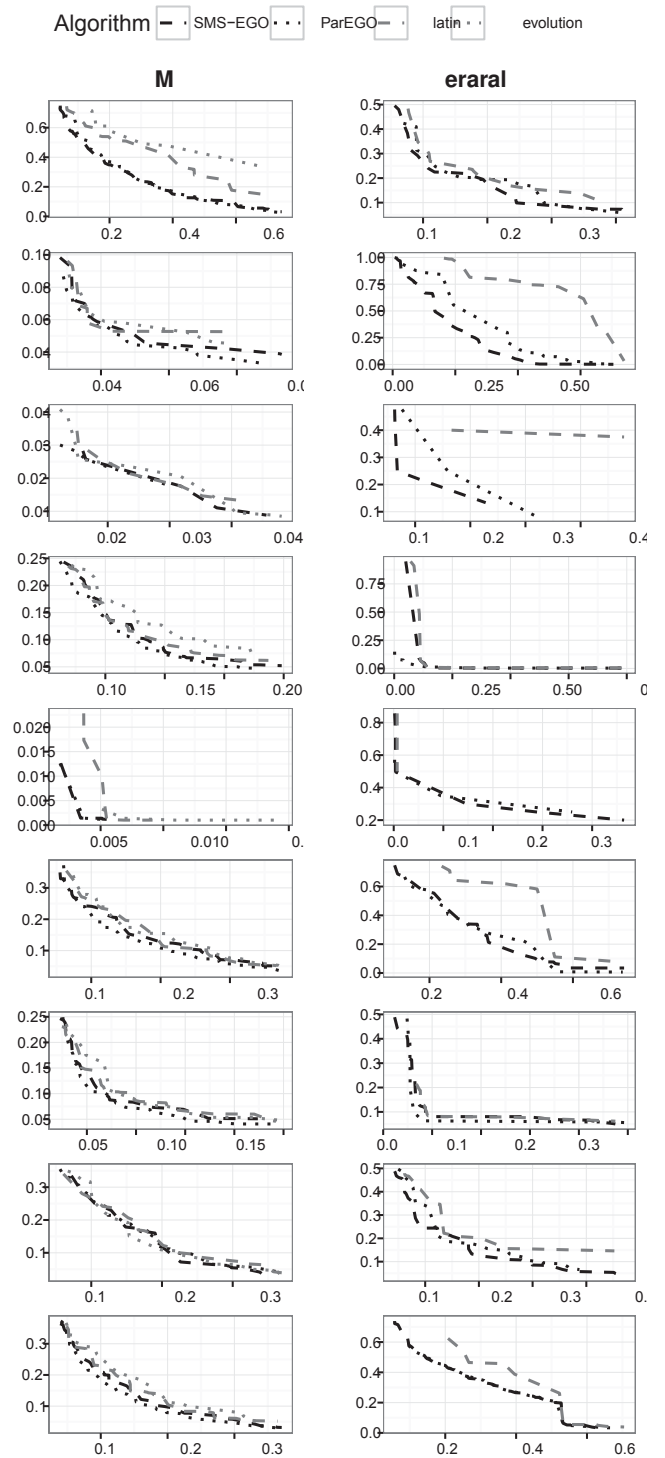
Fig. 3. 50% empirical attainment functions of the two objectives FNR and FPR for both experiments, the axis limits were focused on the interesting parts of the Pareto fronts. The order of the data sets is the same as in Fig. 2.
