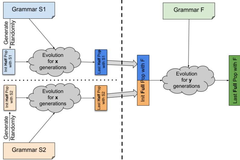
Fig. 3. Overview of the hierarchical grammar approach to G3P using the division of population size strategy with 2 levels (2 small grammars S1 and S2 at the lower level, and one full grammar F at the upper level).
