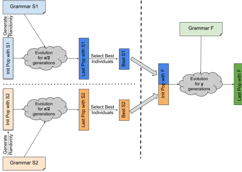
Fig. 2. Overview of the hierarchical grammar approach to G3P using the division of number of generations strategy with 2 levels (2 small grammars S1 and S2 at the lower level, and one full grammar F at the upper level).
