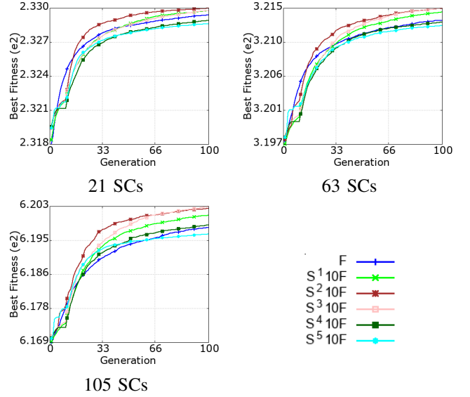
Fig. 4. Average over 30 runs of the evolution of the best fitness obtained by G3P on the different instances with various grammar hierarchies using the division of number of generations strategy.
