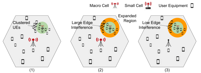
Fig. 1. Example of a Heterogeneous Network with 1 MC, 1 SC, and 21 UEs in three scenarios: (i) with no REB mechanism, (ii) with REB mechanism, and (iii) with REB and muting mechanisms.
