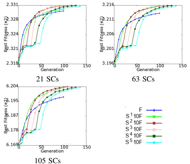
Fig. 5. Average over 30 runs of the evolution of the best fitness obtained by G3P on the different instances with various grammar hierarchies using the division of population strategy. Note that while we have different number of generations for each of the grammar configurations, the computation budget is always the same.
