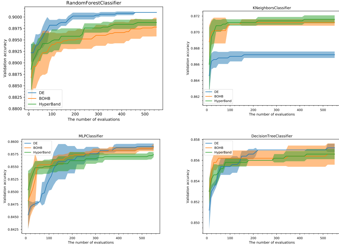
Fig. 5: The convergence plot of the DE, BOHB and Hyperband HPO search strategies over 15 runs. In this figure, the variance of the algorithms is also depicted which indicates how sensitive they are to different random seeds.
