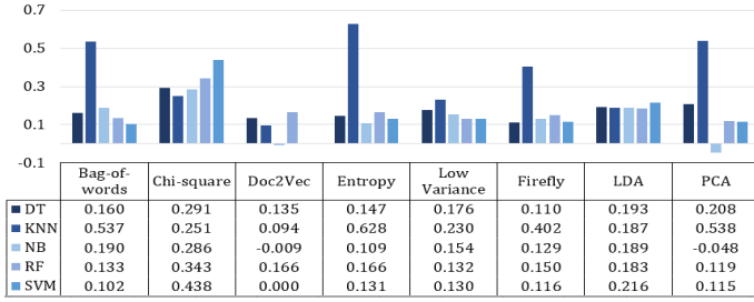
Fig. 3. Impact of proposed method on both classes (F-measure)
